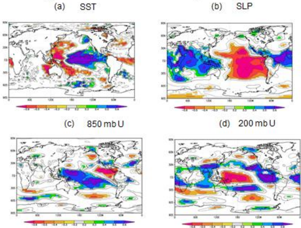
Figure 7: Linear correlations between a 1 March ECMWF SST forecast for September Nino 3 (Predictor 4) and August-October sea surface temperature (panel a), August-October sea level pressure (panel b), August-October 850 mb zonal wind (panel c) and August-October 200 mb zonal wind (panel d). The predictor correlates very strongly with ENSO as well as vertical shear in the Caribbean. The correlation scale has been reversed (sign changed) to allow for easy comparison of correlations for all four predictors.
